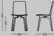
Silla respaldo alto Chair High back
