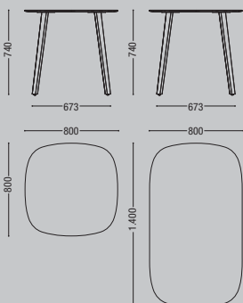
Mesa encimera 800x800mm y 1.400x800mm Table top 800x800mm and 1.400x800mm
